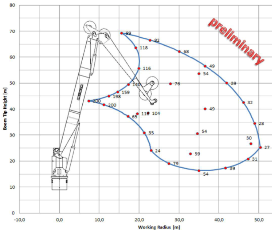
Load chart: Main winch Lift type: Marine / Subsea with AHC
